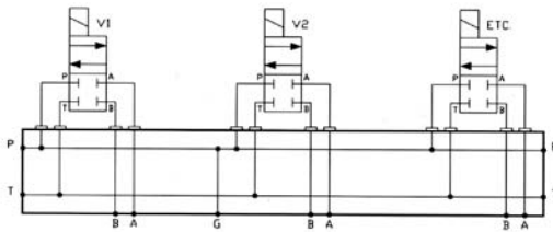
Parallel Circuit
