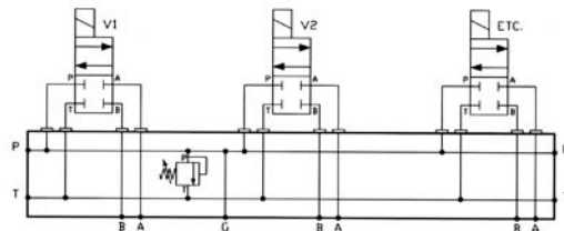
Parallel Circuit with relief
