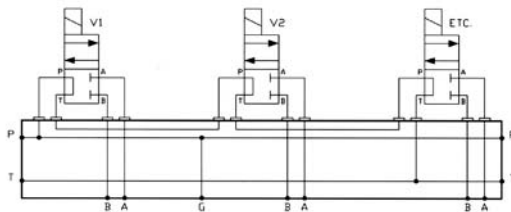
Series Circuit
