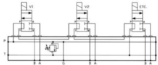
Series Circuit with relief
